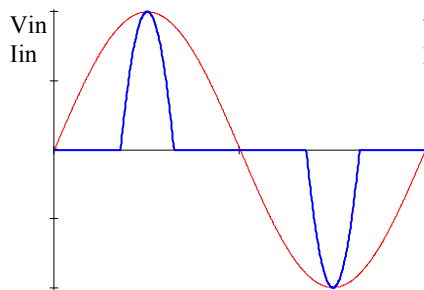
Figure 2: Typical input current without harmonic line current reduction
